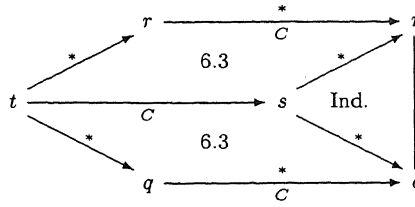
Figure 9. Proof of preservation of UN^\rightarrow .
